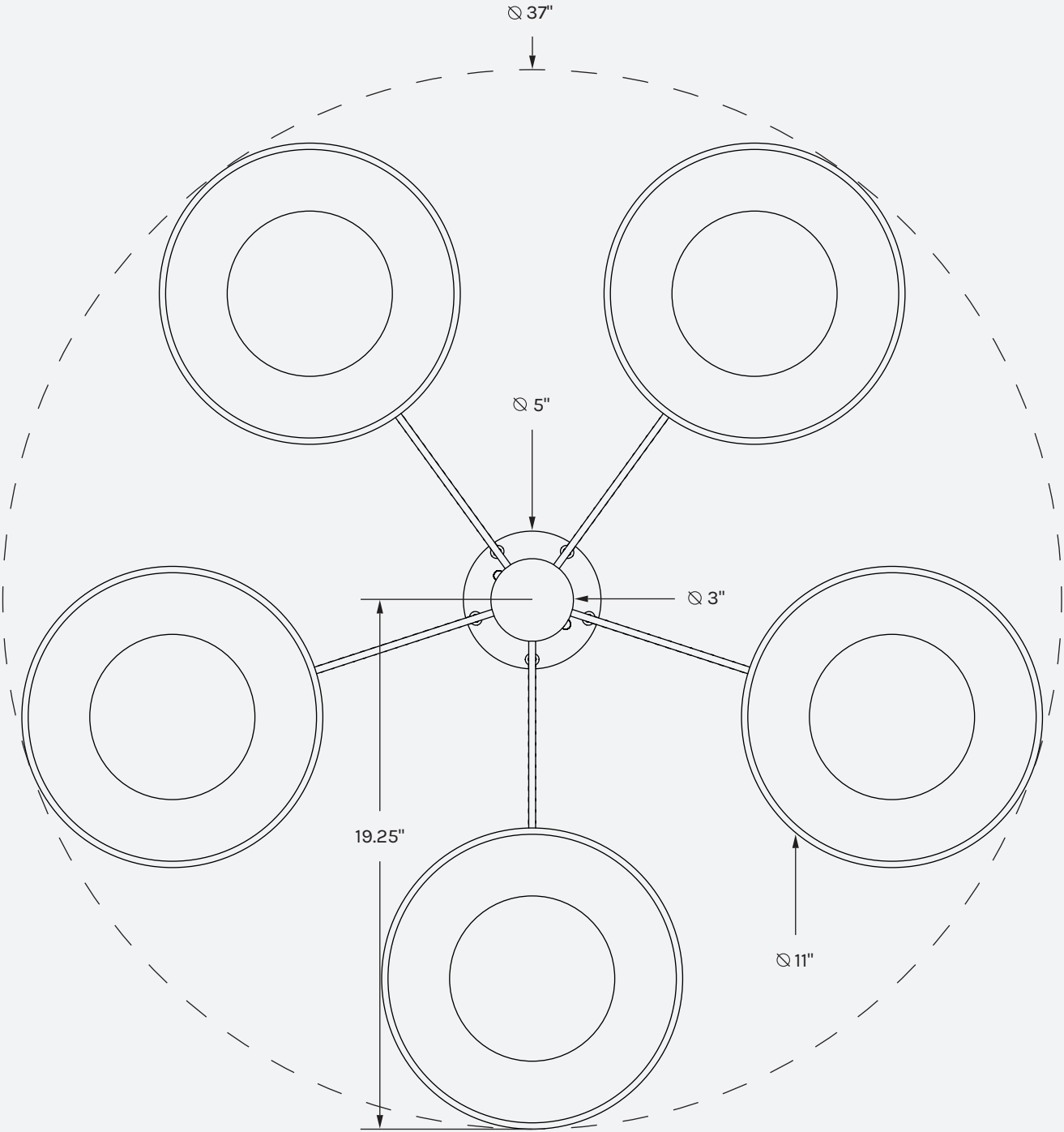
BOTTOM VIEW
